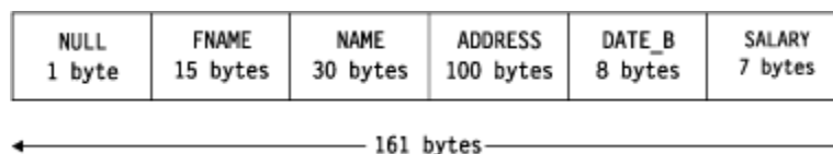
Figure 13. Output record format: sequential data set in USER format
